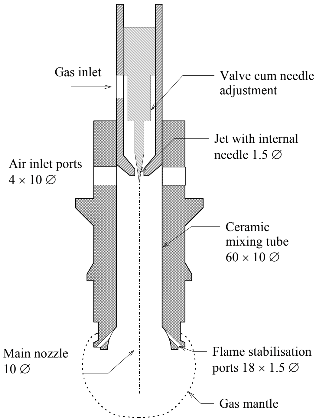
DCS gas lamp burner design
